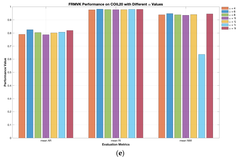
Figure 6. The Clustering performances of three related algorithms on COIL20 data based on different tuning parameters: (a) WMCFS under different \beta and fixed \alpha = 7 ; (b) WMCFS under fixed \beta = 0.005 and different \alpha ; (c) SWVF under fixed \alpha and different \beta ; (d) SWVF under fixed \beta and different \alpha ; (e) FRMVK under different \alpha .
