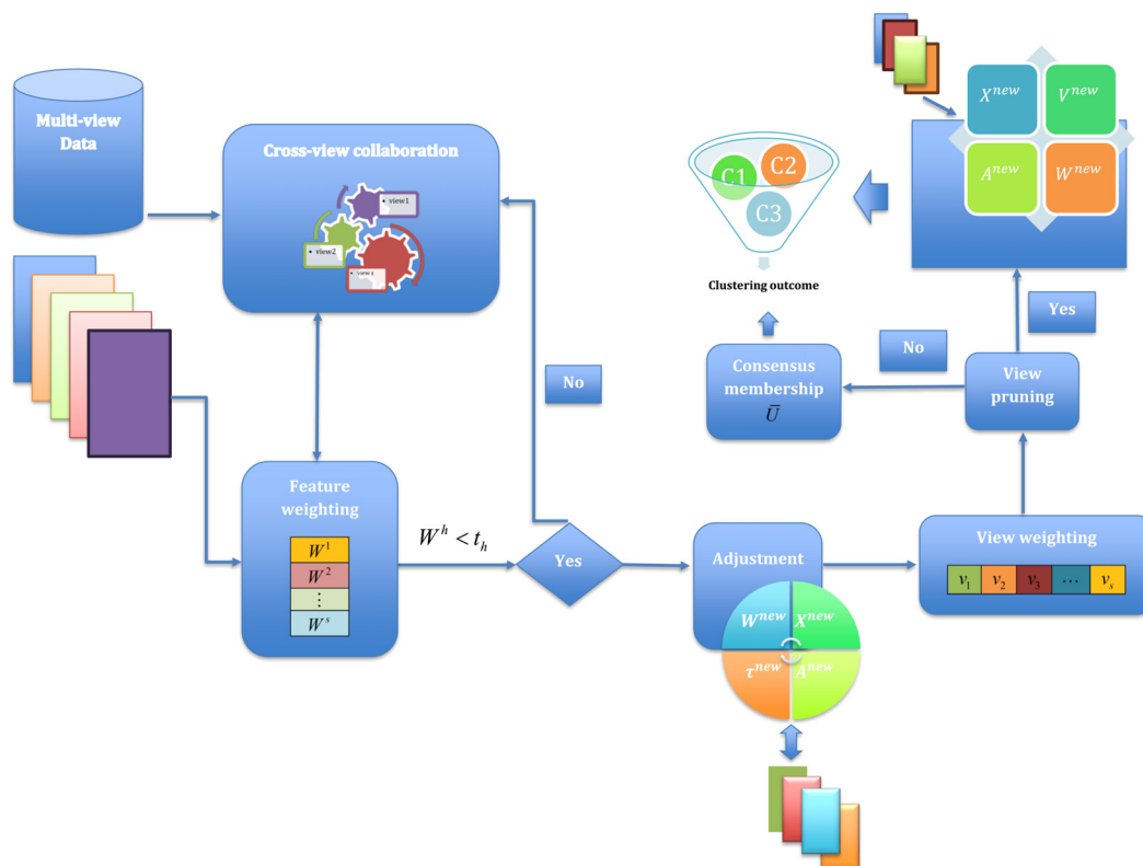
Figure 1. Overall architecture of the proposed G-CoMVKM.
