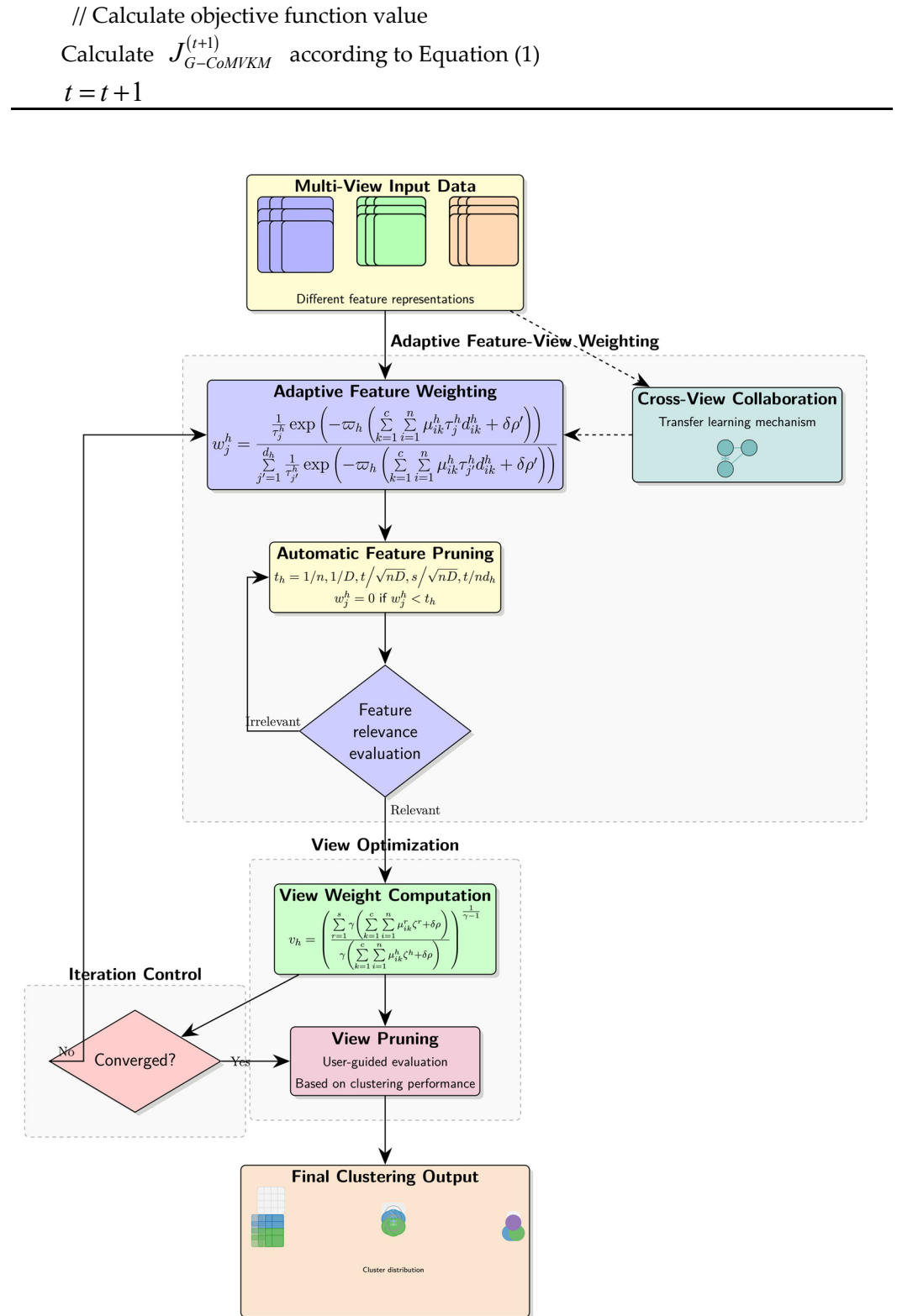
Figure 2. Flowchart of the proposed G-CoMVKM algorithm.
